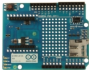
Arduino Wireless SD Shield
