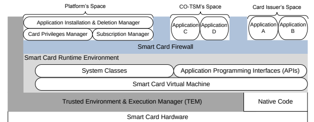
Figure 6. Smart Card Architecture
